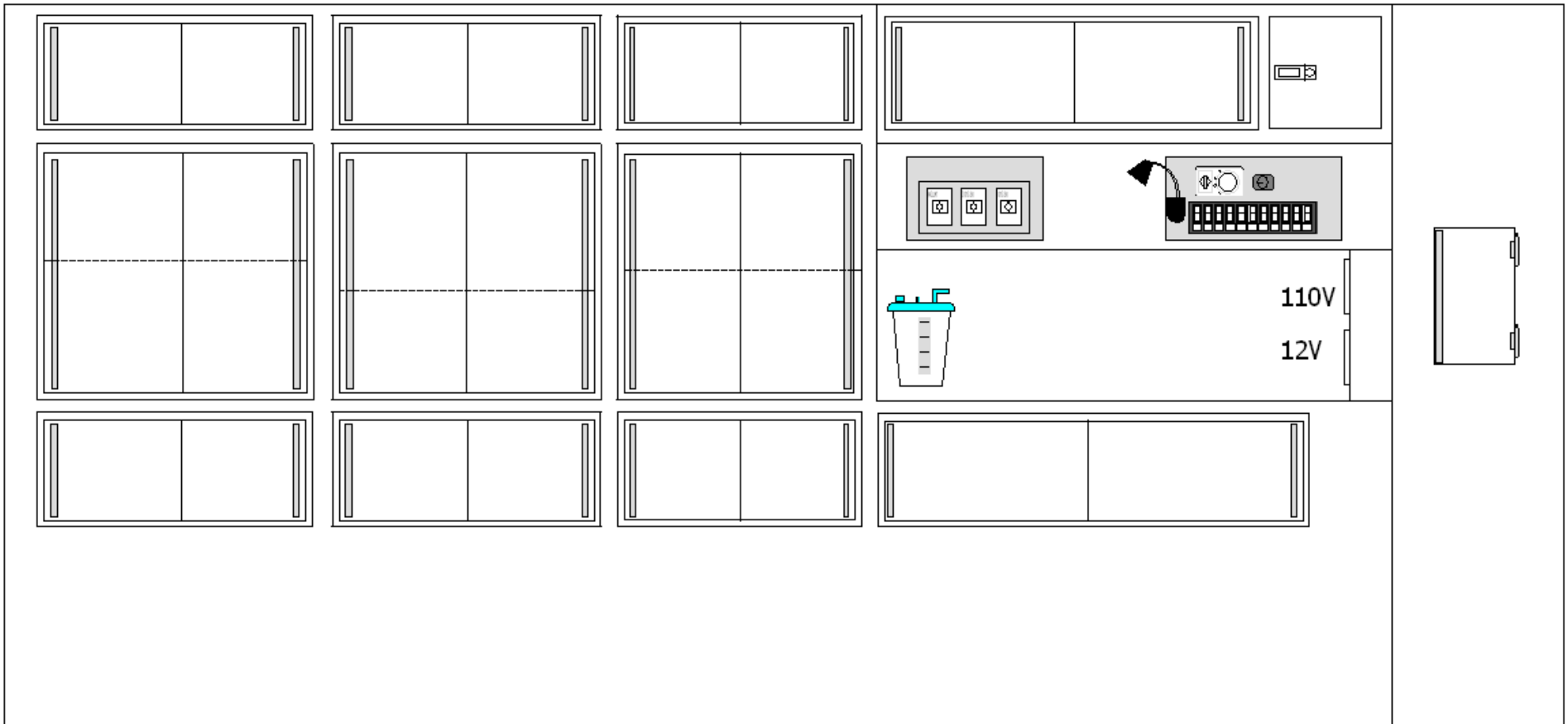
TAYLOR MADE AMBULANCE FORD TYPE I F-350 150" MODULE 68" HEADROOM LEFT WALL #1 2009
