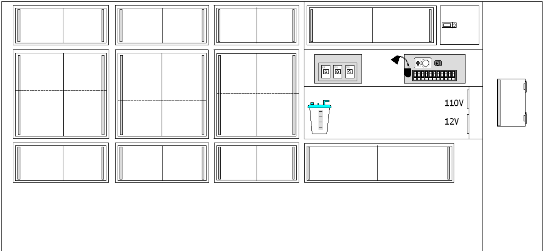
TAYLOR MADE AMBULANCE FORD TYPE I F-450 150" MODULE 68" HEADROOM LEFT WALL #1 2009
