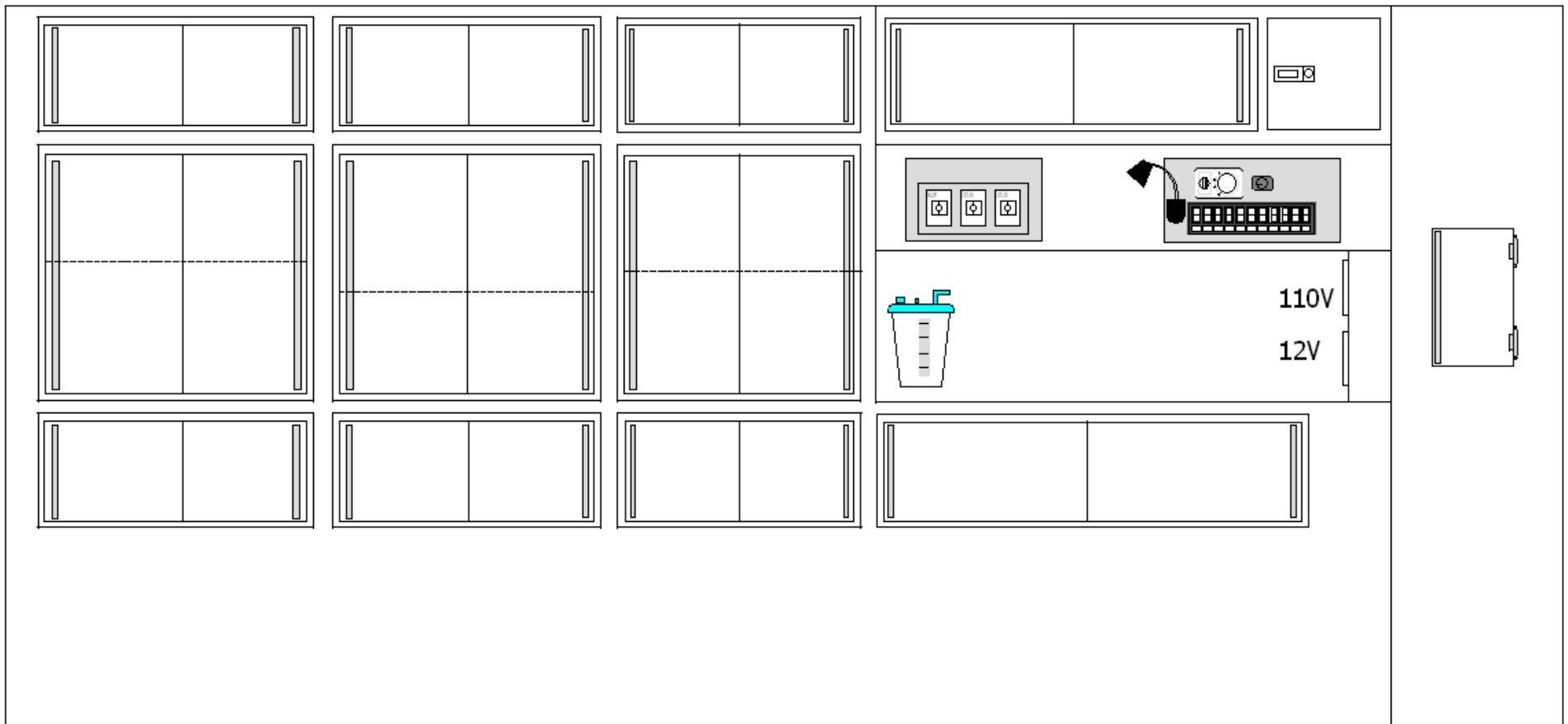
TAYLOR MADE AMBULANCE FORD TYPE I F-450 150" MODULE 72" HEADROOM LEFT WALL #1 2009
