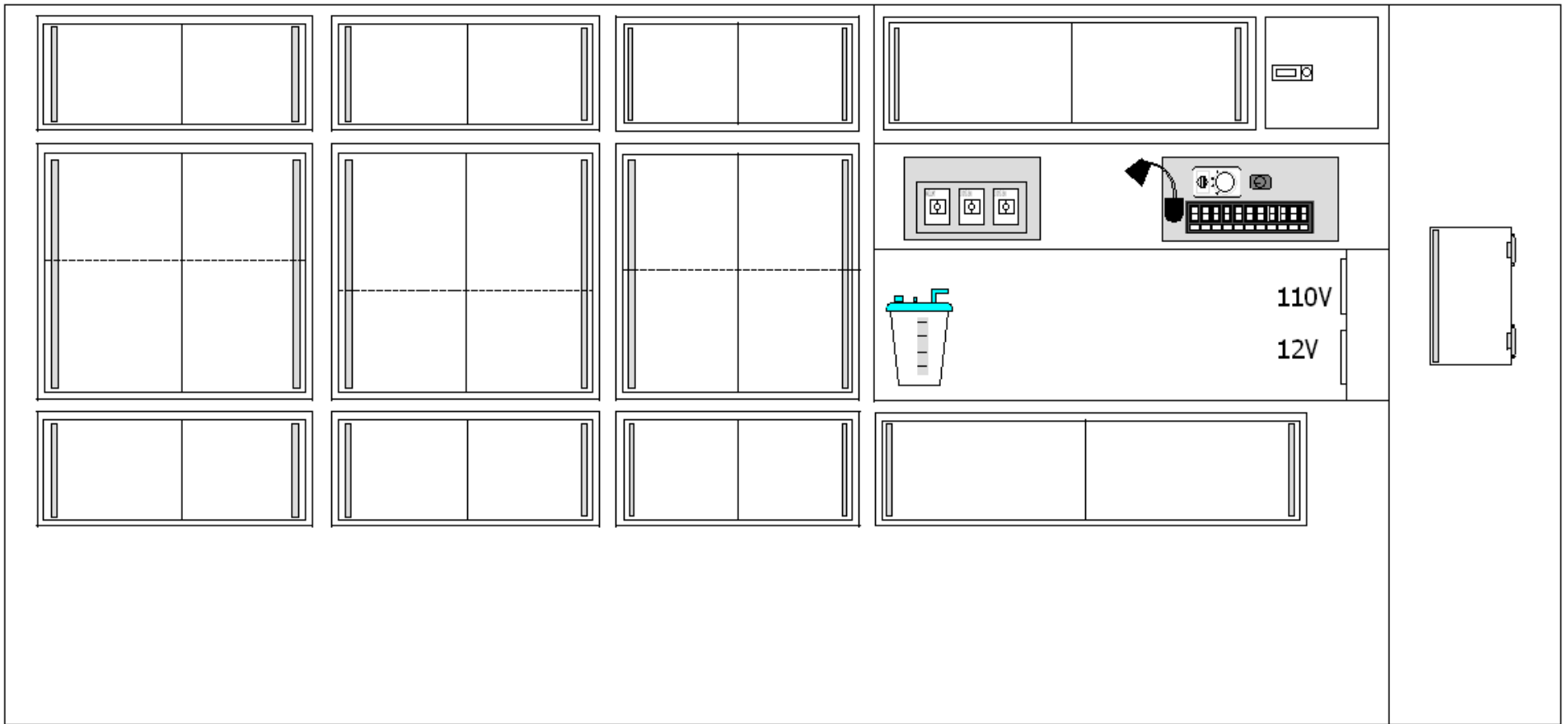
TAYLOR MADE AMBULANCE FORD TYPE I F-550 150" MODULE 72" HEADROOM LEFT WALL #1 2009
