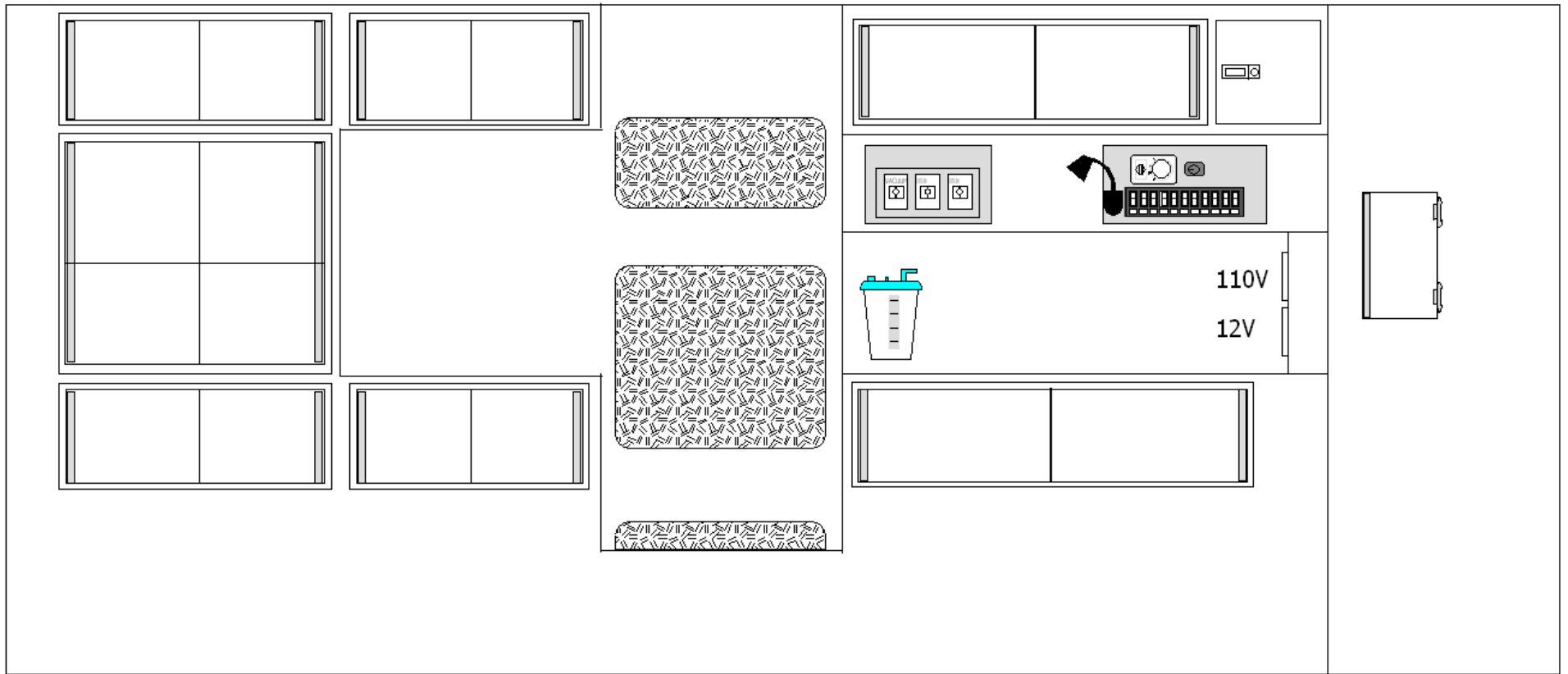
TAYLOR MADE AMBULANCE GM 4500 TYPE I 164" MODULE 72" HEADROOM LEFT WALL #3 2009
