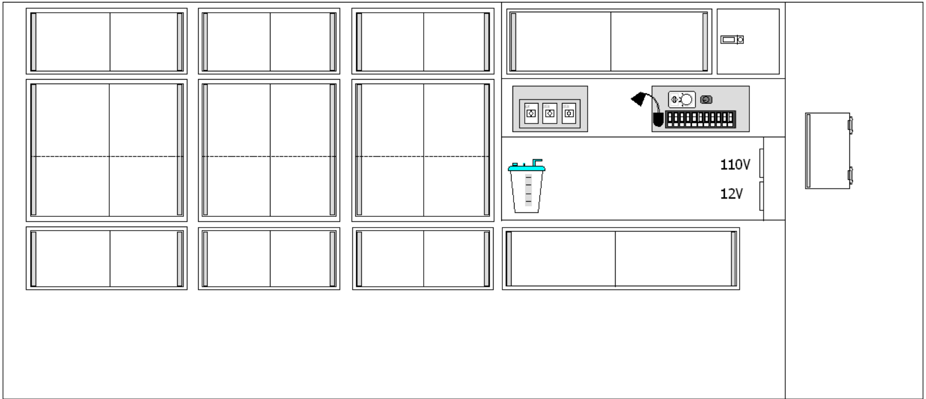
TAYLOR MADE AMBULANCE INTERNATIONAL TYPE I 164" MODULE 72" HEADROOM LEFT WALL #1 2009
